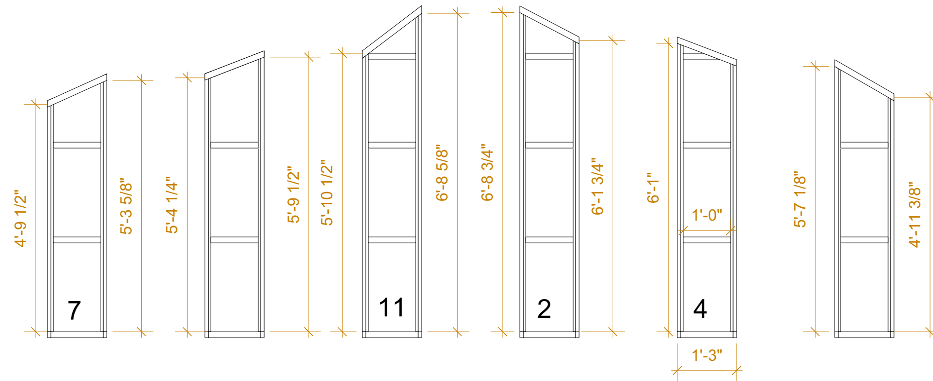
1 Tree Trunk Detail Scale: 1/2" = 1'-0"
